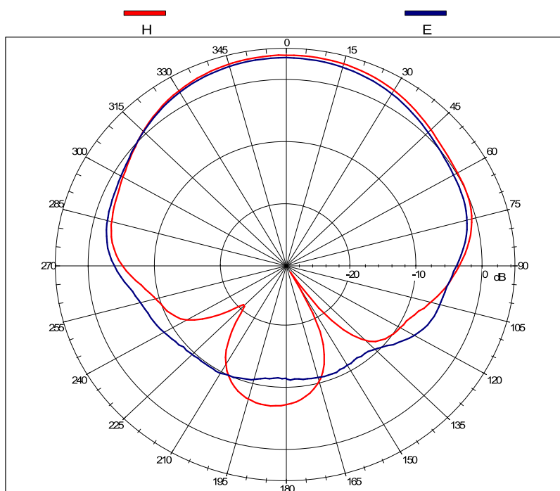
Right hand circular polarized signal f_0=1606\text{MHz}
