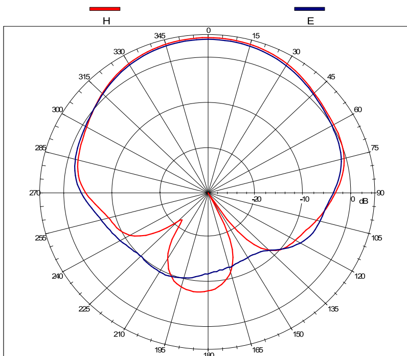
Right hand circular polarized signal f_0=1602\text{MHz}
