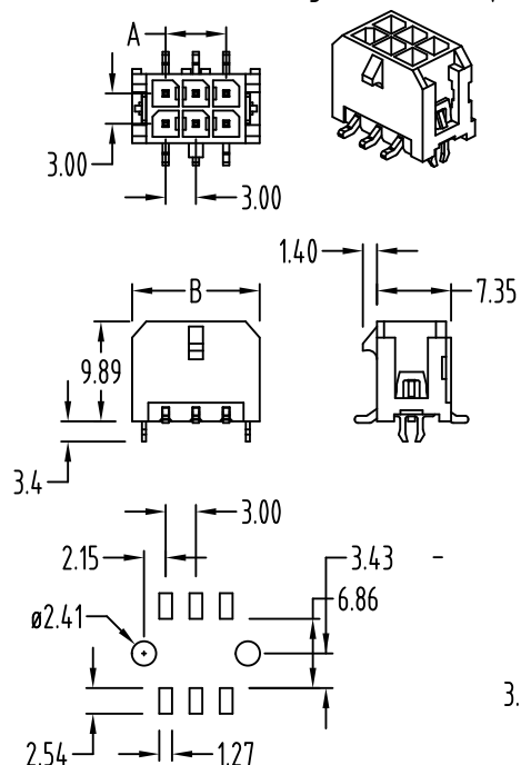
S30002-HA2-XX-X (With Soldering Retention Clipse)
