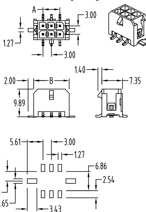
S30002-HC2-XX-X (With Soldering Fitting Nail)
