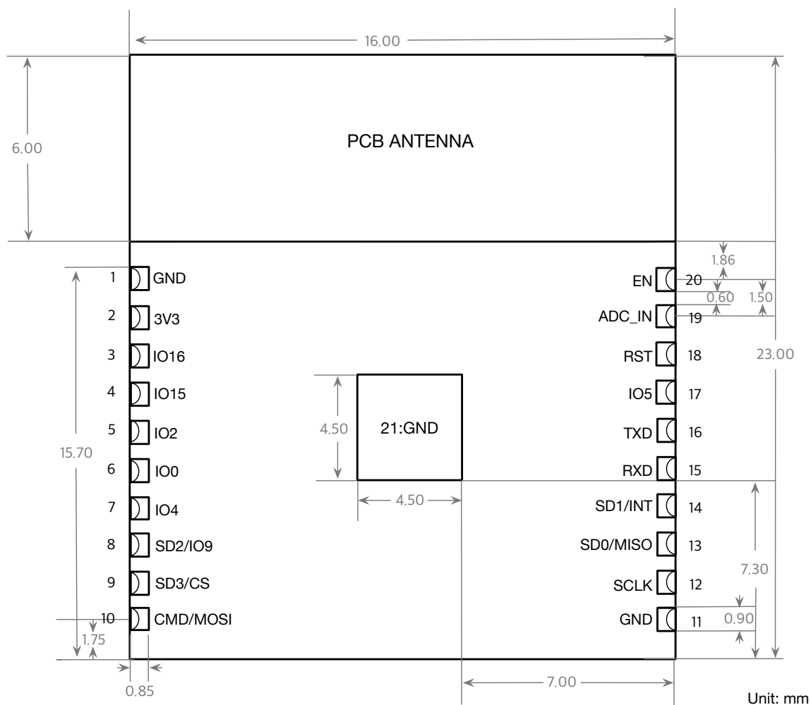
Figure 2-1. ESP-WROOM-S2 Pin Layout (Top View)
