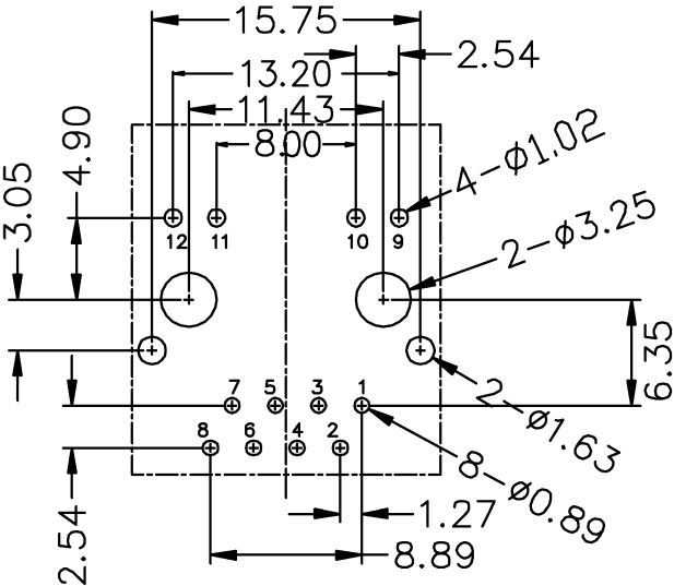
RECOMMENDED P.C.B.LAYOUT ALL TOLERANCES ARE±0.05
